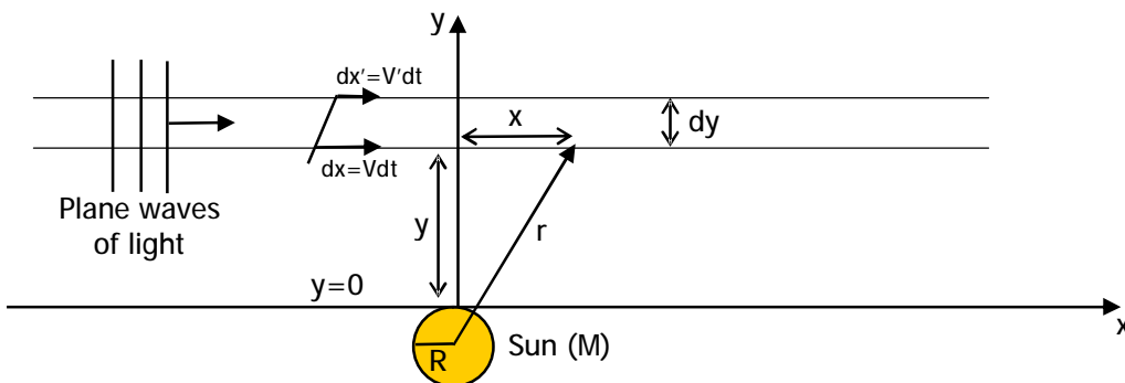
Fig. 2: Drawing for calculations.
