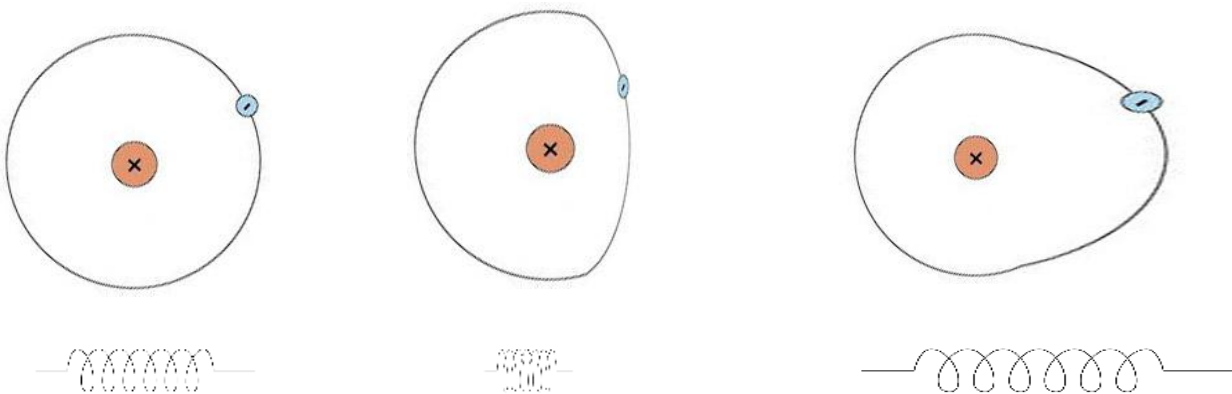
Fig. 3.1: H Atom (normal, compressed and expanded).
