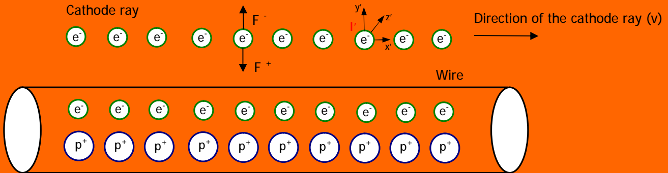
Fig. 1.3: Wire not flown by any current, seen from the cathode ray steady ref. system \bar{I} ( x', y', z' ).
