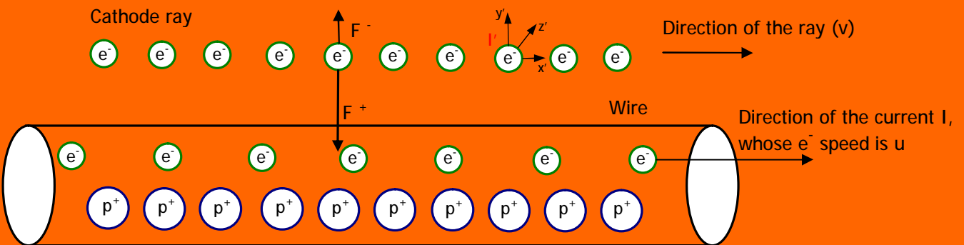
Fig. 1.4: Wire flown by a current (with e^- speed= u ), seen from the cathode ray steady ref. system \bar{I} ( x', y', z' ).
